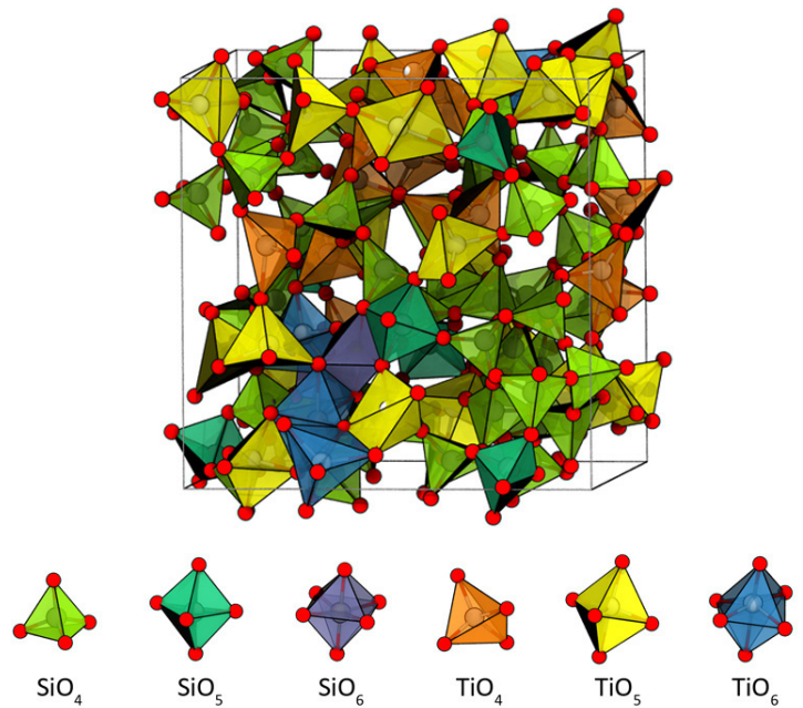
Calculated geometry of amorphous Ti_{0.4}Si_{0.6}O_2 in coordination polyhedra representation.
