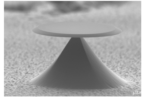
Silicon oxinitride microresonator on a silicon substrate
