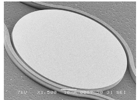
Waveguide coupled microresonator based on silicon oxinitride
