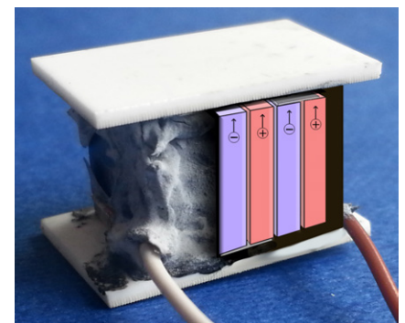
Thermoelectric generator with titan silicide contacts
