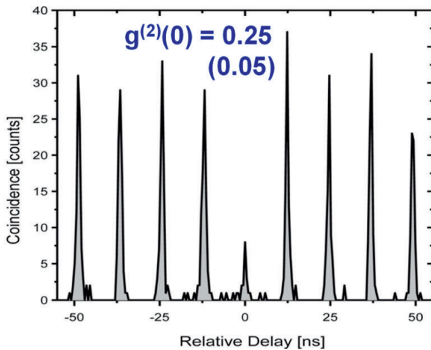
Fig. 2: Autocorrelation histogram of a single c-GaN QD emitting at 3.687 eV at 4 K. The excitation power was 20 mW and the PL decay time is about 360 ps. The number in the bracket is the background corrected value of g^{(2)}(0) .
