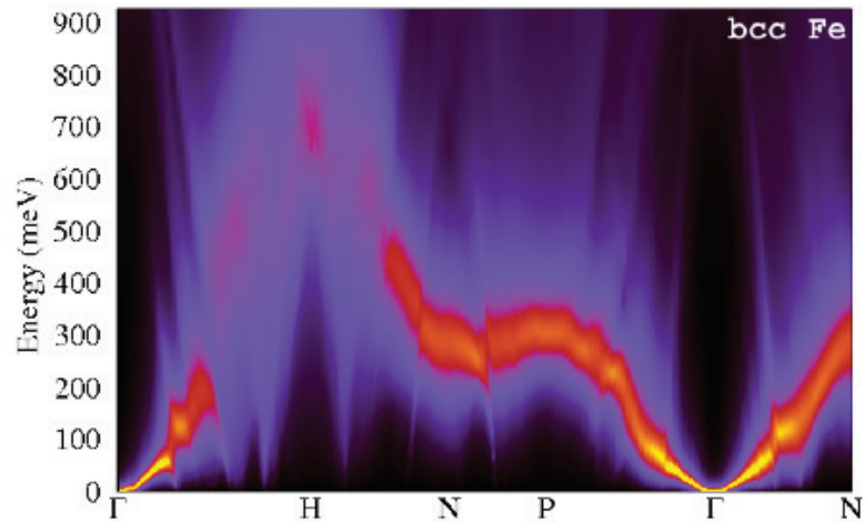
Calculated spin-wave dispersion of iron.
