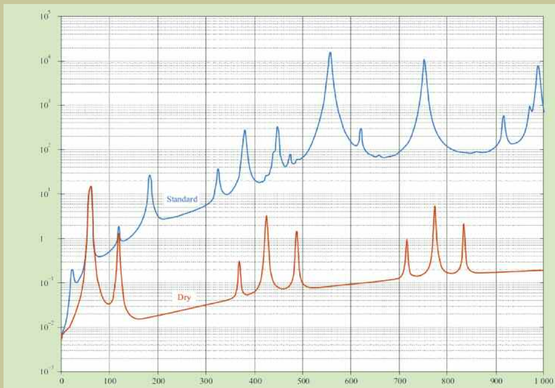
Fig. 1: Frequency-dependent attenuation by molecules in the atmosphere [3].
