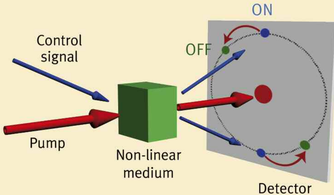
Fig. 1: Simplified illustration of a switching process based on optical patterns in a non-linear medium. The figure shows the ON state. When the control signal is switched off, the system and the detected signal revert to the OFF state.
