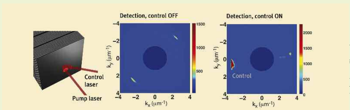
Fig. 4: Experiment on switching with patterns. Data from [4].
