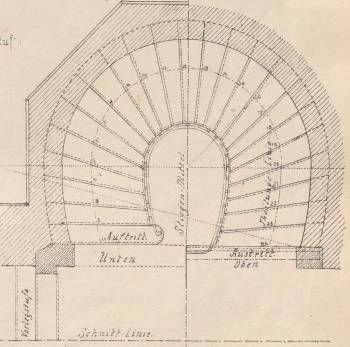
Grundriss in Kuffenform
