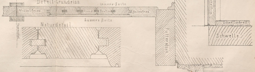
Detail-Grundriss.
