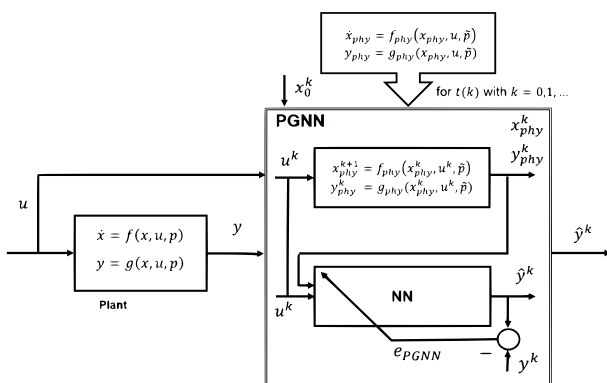
PGNN während des Trainings PGNN during training
