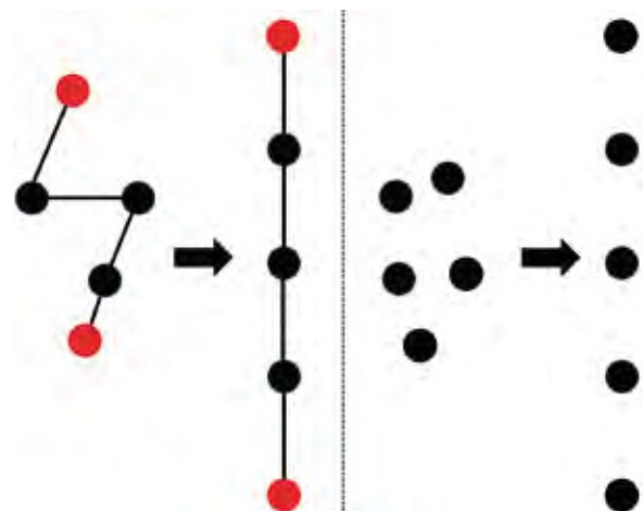
Das Max-Chain-Formation-Problem (links) und das Max-Line-Formation Problem (rechts). The Max-Chain-Formation problem (left) and the Max-Line-Formation problem (right).
