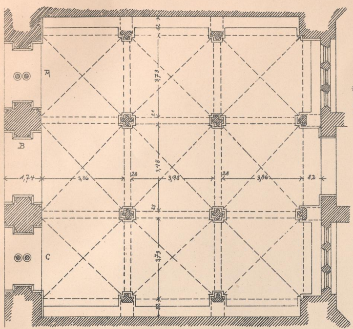
GRUNDRISS = 1:100
