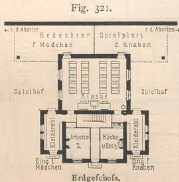
Erdgeschofs.
