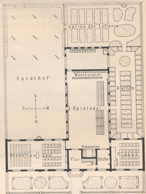
Erdgechofs.
