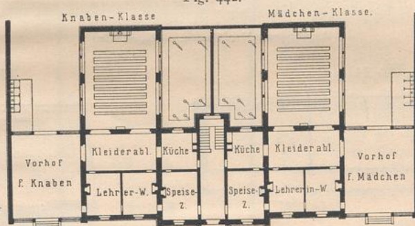
Erdgeschoss.
