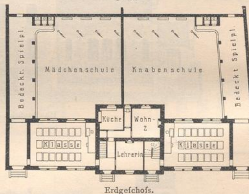
Erdgechofs.
