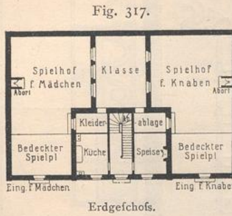
Erdgeschofs.
