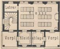
Erdgeschoss.
