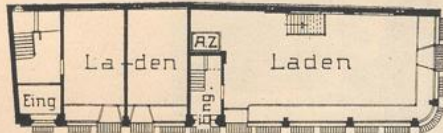
Erdgeschoss.
