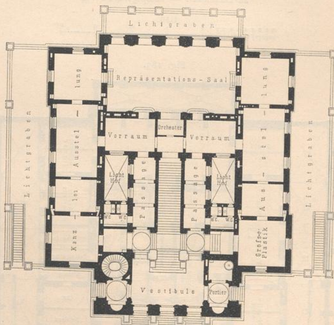
Erdgefchofs.
