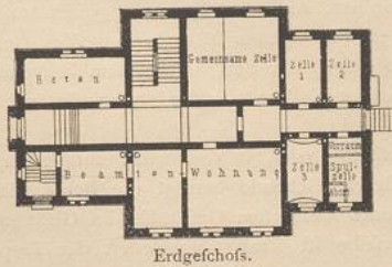
Erdgeschoss.
