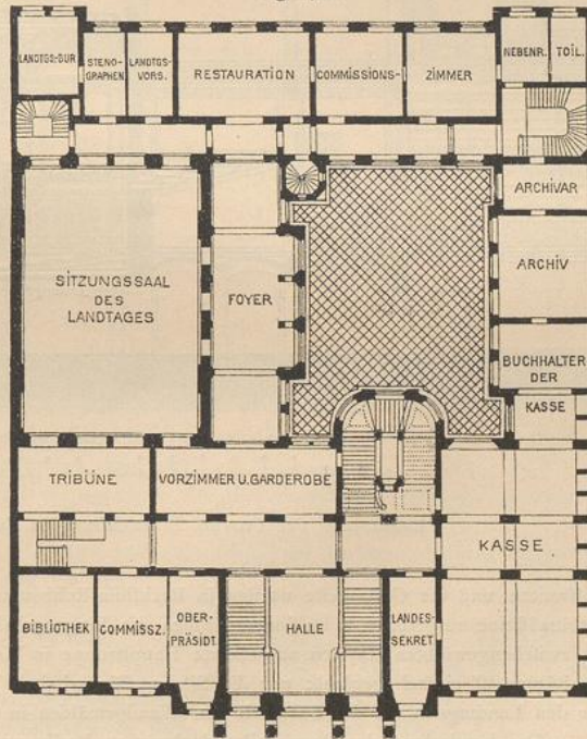
Erdgeschoss.
