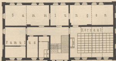
Erdgeschoss.
