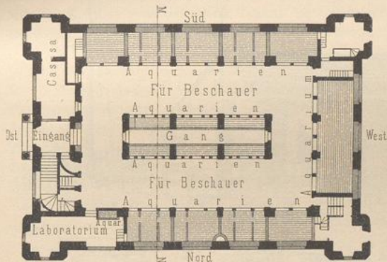
Erdgefchofs.
