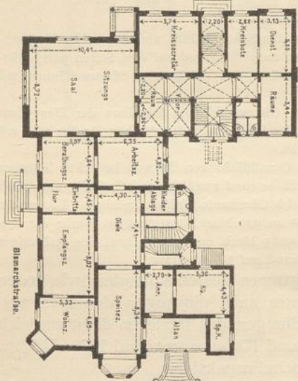
Erdgeschoss.
