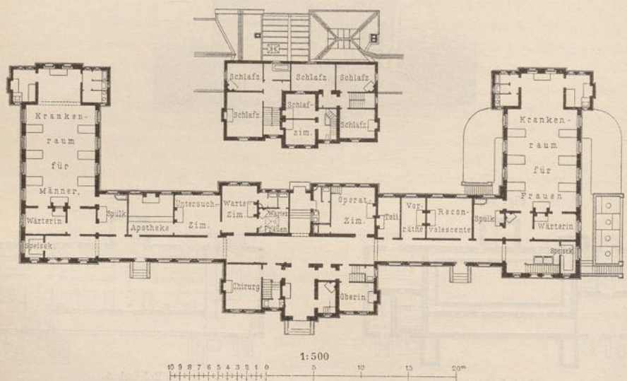
Horton infirmary zu Banbury 1749 .
