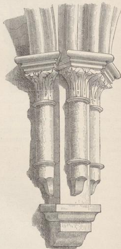
Fig. 445. Wandpfeiler aus Maulbronn. (C. Riefs.)
