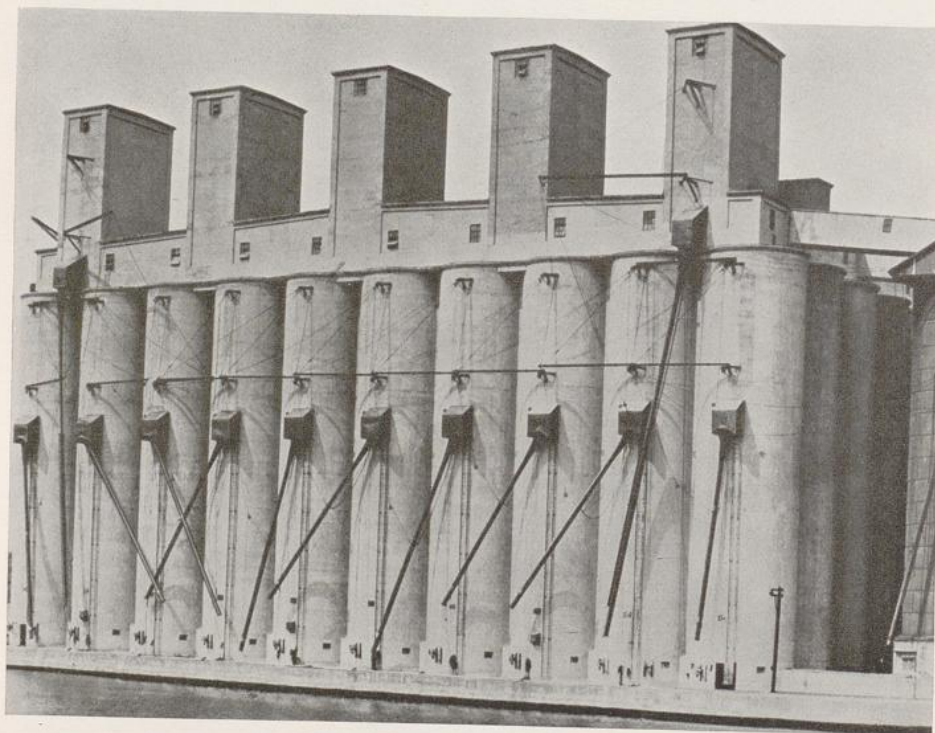
Getreidesilos, Fort William (Ontario, Canada). 1914
