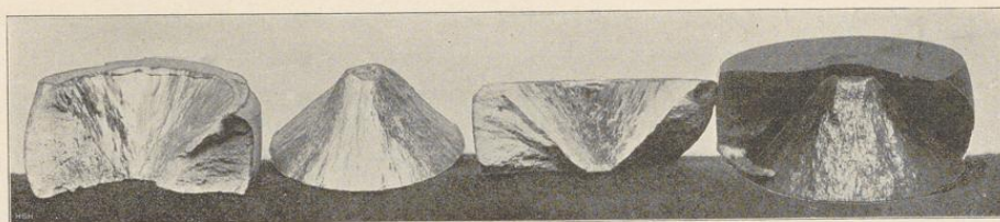
Stauchversuch.
