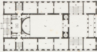
Grundriß oberer Stock
