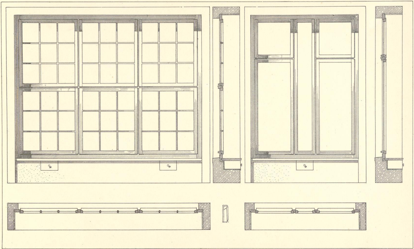
Fenster.
