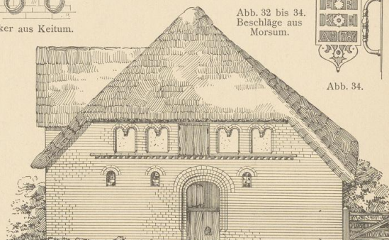
Abb. 12. Haus Hansen in Klockries, 1634. 1:100.
