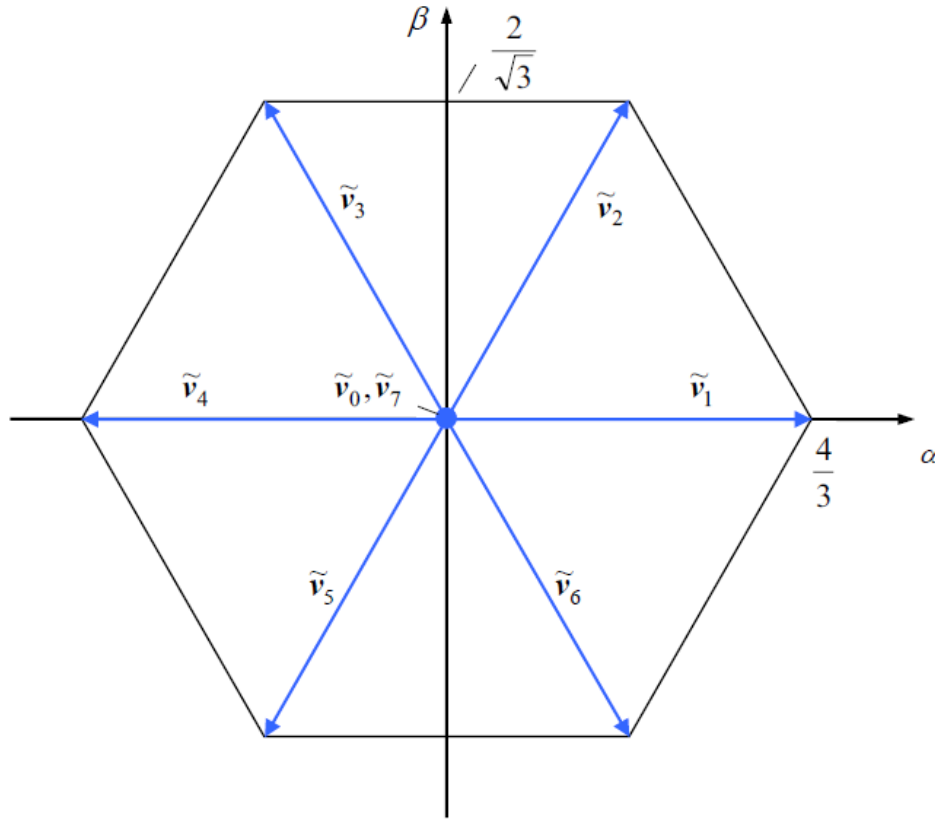
Fig. 2.4: Normalized switching vectors of the inverter [2]
