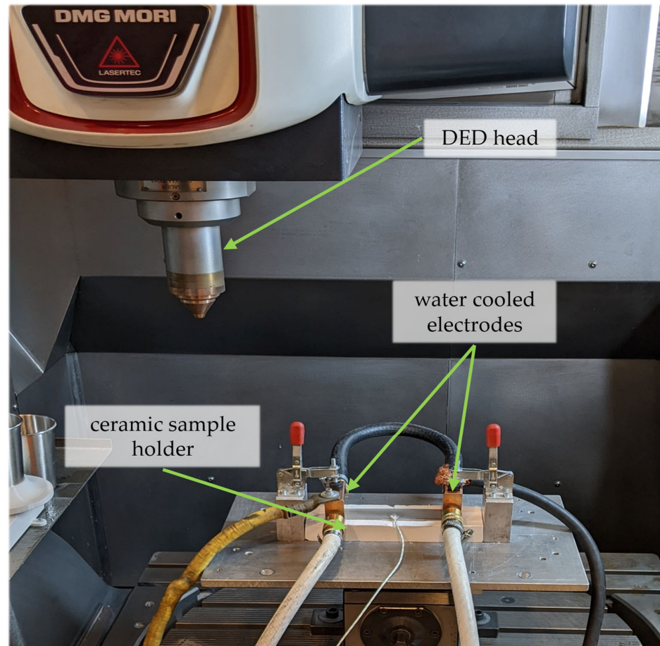
Figure 2. Sample production setup.
