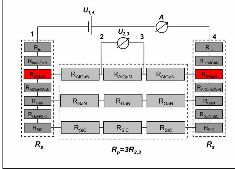
Figure 3.19: Equivalent current circle of the investigated AlGaN/GaN samples.
