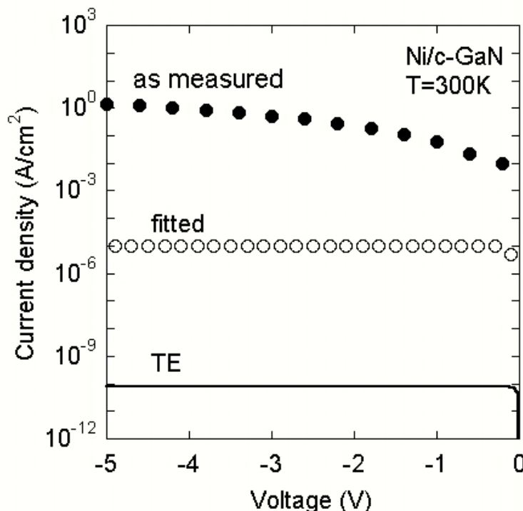
Figure 4.9: Comparison of the measured I-V curve (full circles), eliminating the influence of R_S (open circles) and the calculation using the Schottky-Mott equation (solid line) in reverse direction for GNJ1204.
