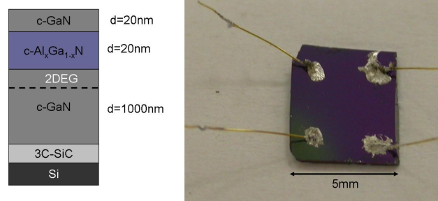
Figure 6.22: Structure and photograph of the AlGaN/GaN heterostructure which is used for the Hall-effect analysis.
