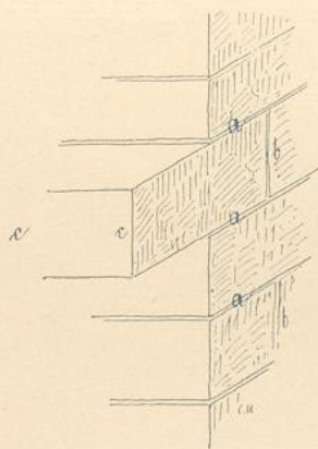
Fig. 99. Steinverband.
